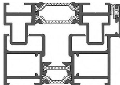
Frame jamb section (with adjustable jamb attached)
