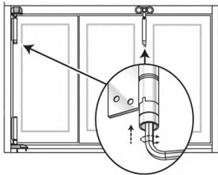
FIG A: ALLEN KEY ADJUSTMENT METHOD
