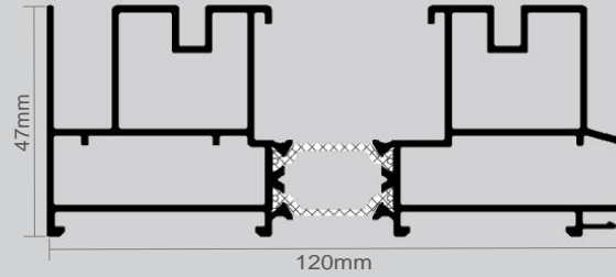
FRAME JAMBS/ HEAD/ BOTTOM TRACK
