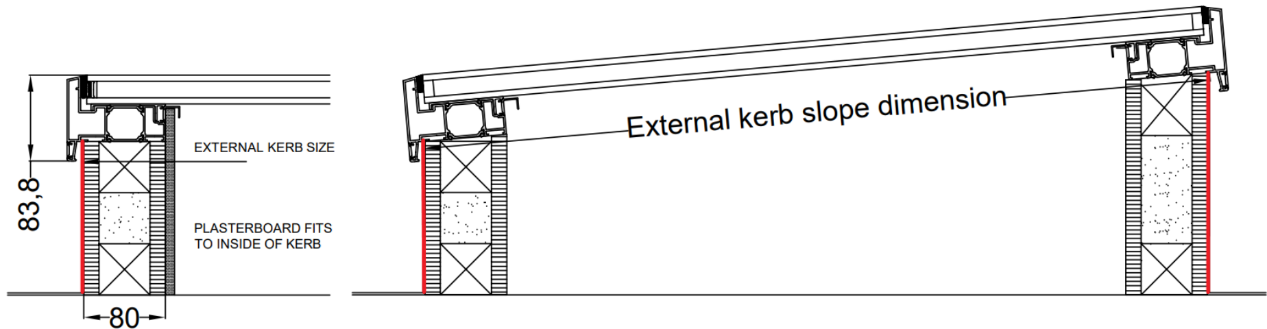
SIDE ELEVATION
