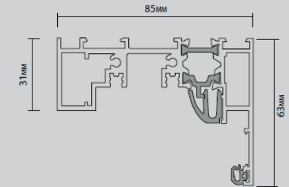
FRAME HEAD
