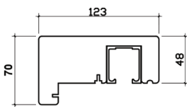
FRAME HEAD
